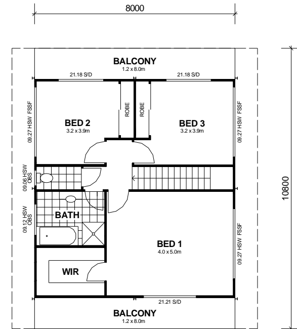
SECOND FLOOR
