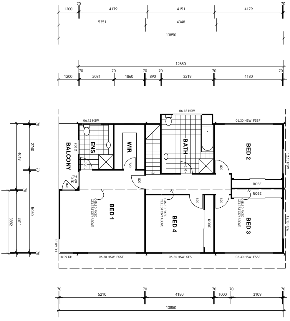
SECOND FLOOR
